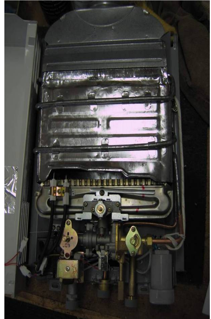
Front view w/o cover
